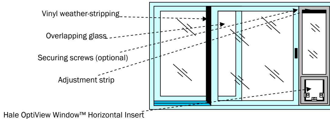
Figure 3 Installed horizontal Hale OptiView Window™ model
